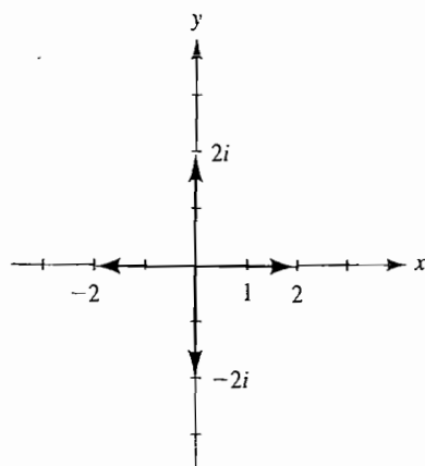
FIGURE 9.10 The fourth roots of 16.
